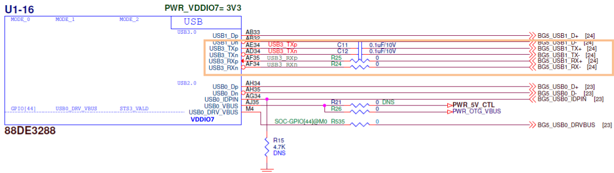
Figure1: USB3.0 connector circuit of EVB.
