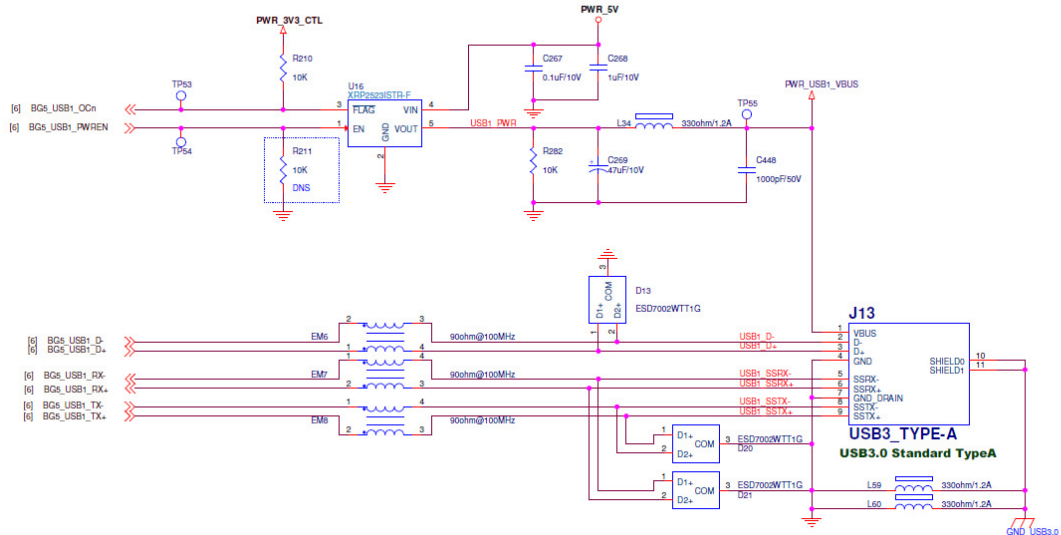
USB3.0 Connector Circuit
