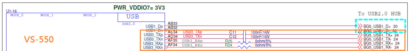
Figure1: USB3.0 connector circuit of BFX-UA300.
